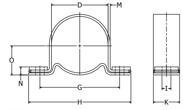
BK Brackets
