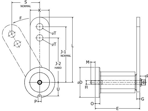
Tensioners Type SE-F (for use with metric Idler Hardware)
