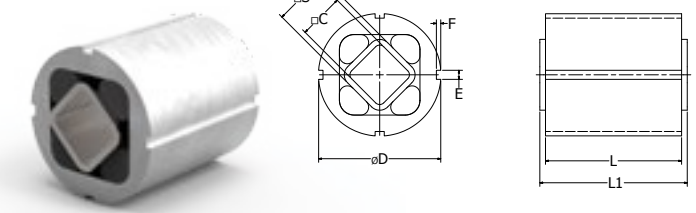
Rubber Suspension Units DK-A, DK-S
