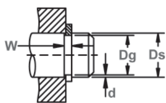
Shaft Diameter & Groove Dimensions
