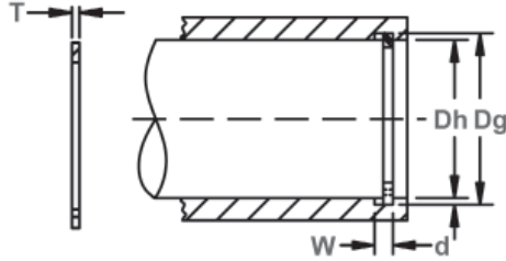
Housing Diameter & Groove Dimensions
