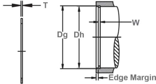
Housing Diameter & Groove Dimensions
