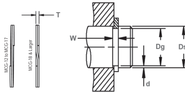
Shaft Diameter & Groove Dimensions
