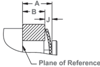
Outer Groove Location A \text{ max} = B \text{ min} + J \text{ max} A \text{ min} = B \text{ max} + J \text{ min}
