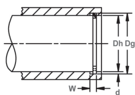
Housing Diameter & Groove Dimensions
