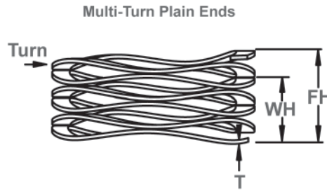
Wave Spring Measurements
